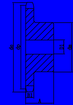
A型叁排平片链轮 A type triplex plate wheels
